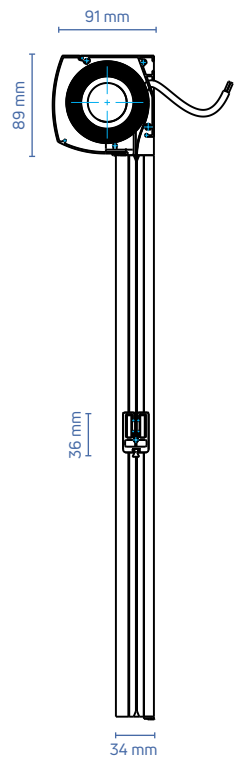
Section view
