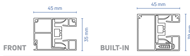
Guide rails
